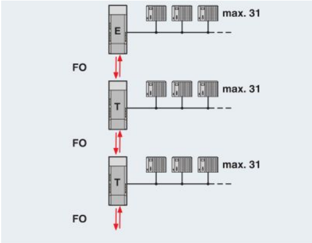
Application drawing
